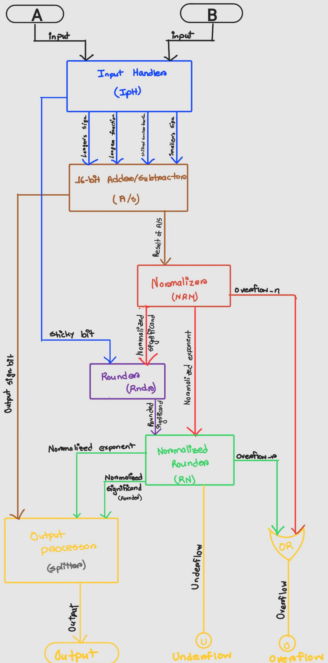
Fig Block Diagram of FPA
